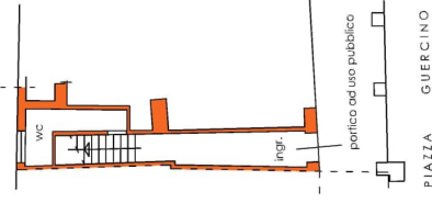
PIANO TERRA
