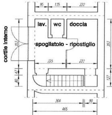
PIANO TERRA H. 270 SPOGLIAT. / RIP. - PARTIC. 1409 SUB. 4
