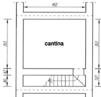
PIANO INTERRATO H. 250 CANTINA - PARTIC. 1409 SUB. 4
