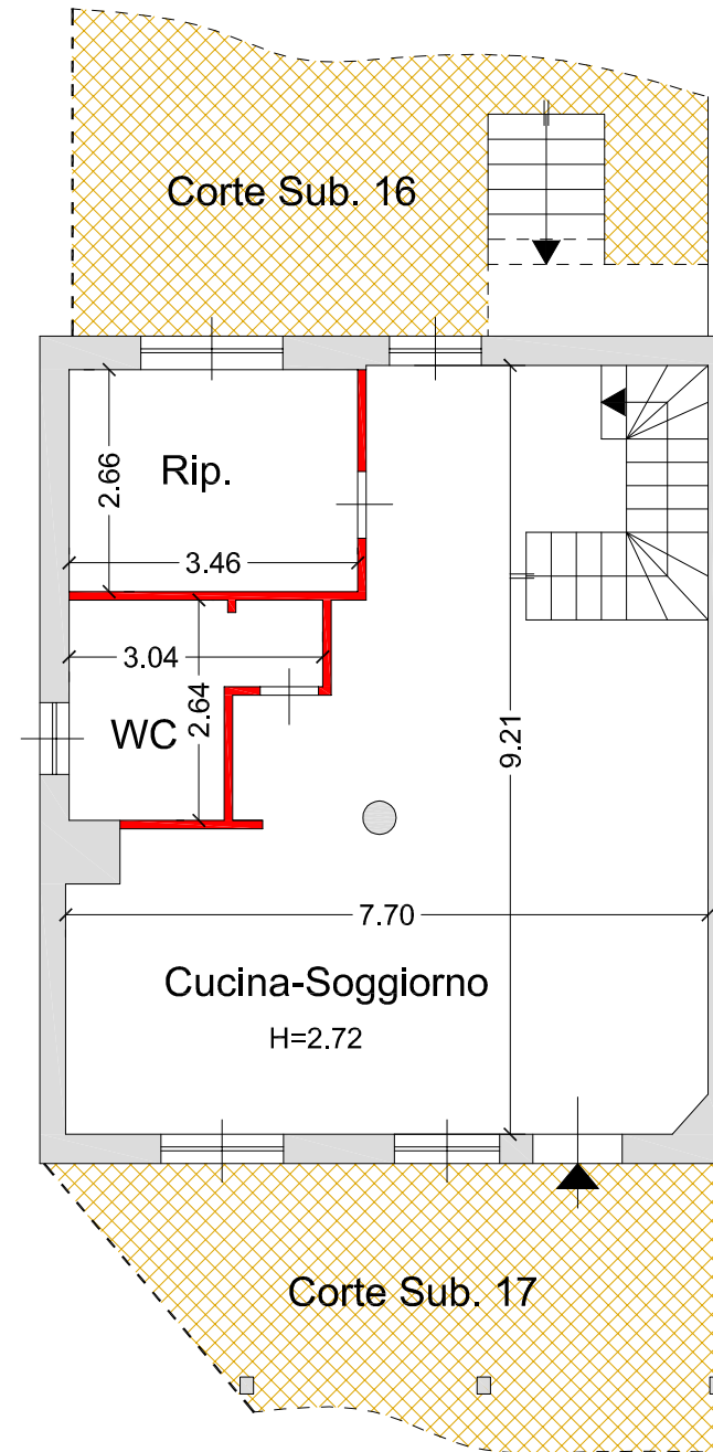
Piano Terra
