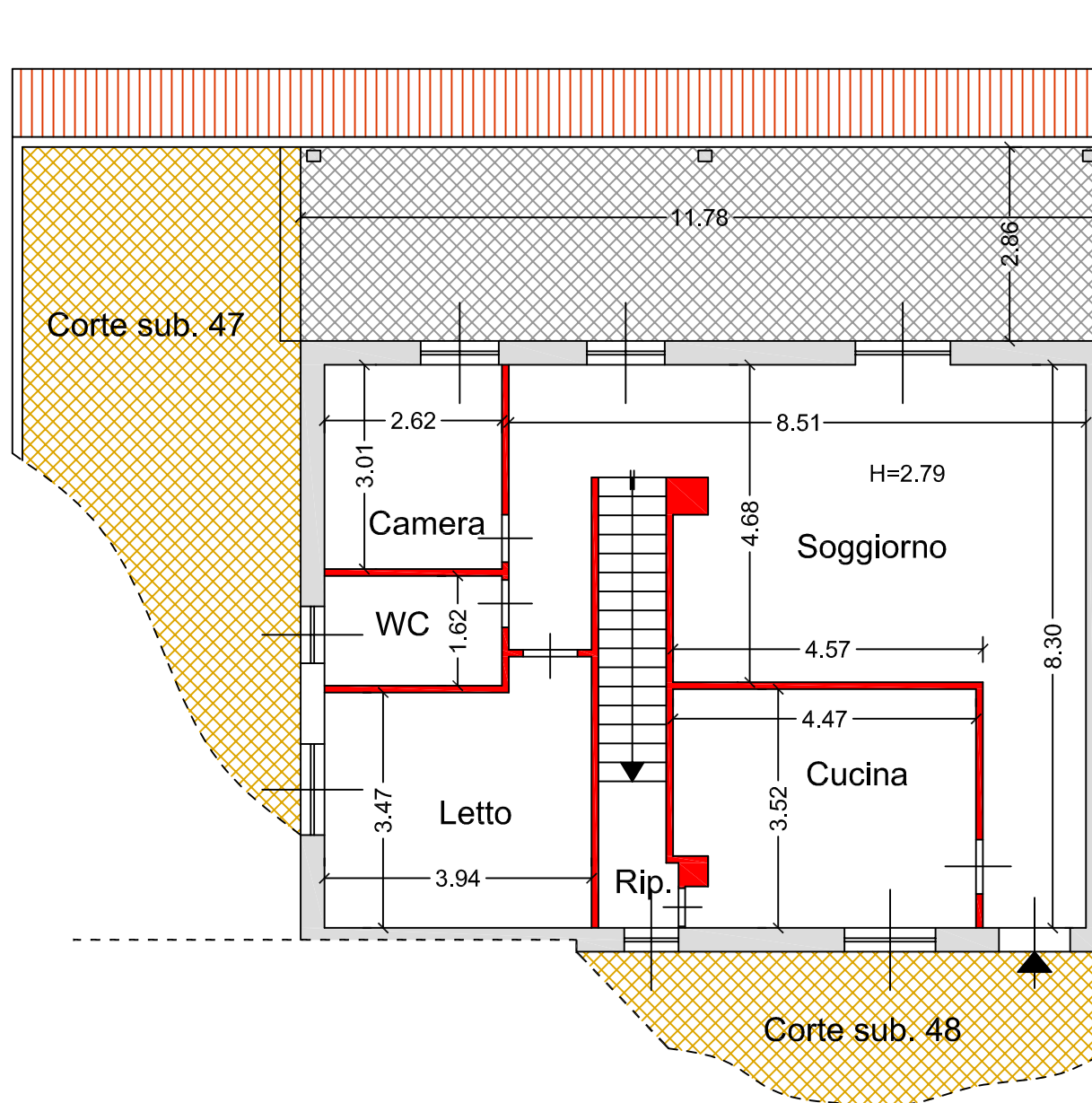
Piano Terra
