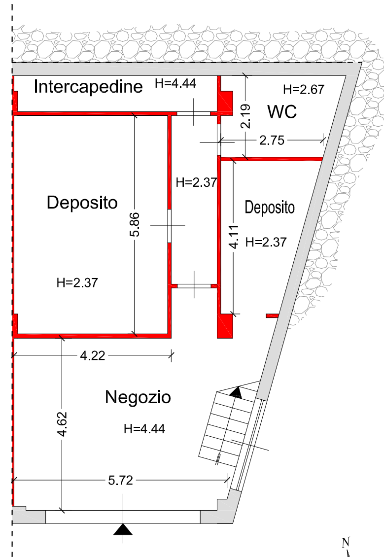
Piano Seminterrato
