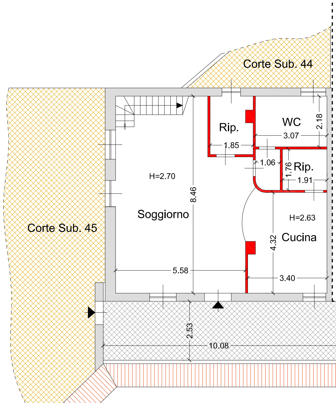
Piano Terra
